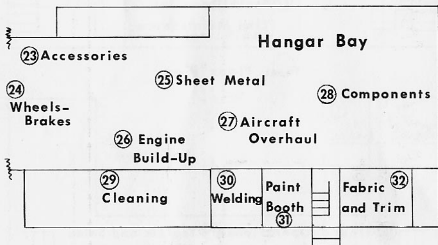
First Floor Plan, South half
